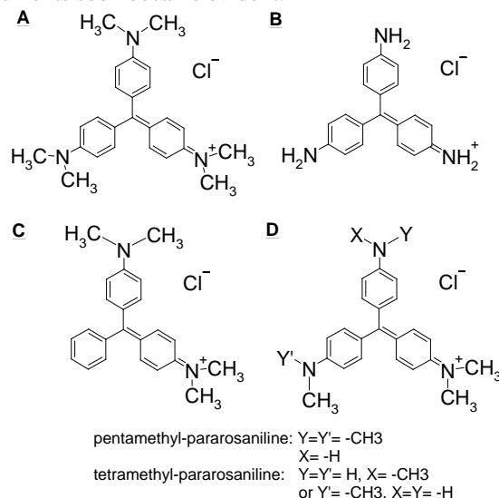
Figure 1: molecular structures for CV (A), pararosaniline (B), diamond green B (C) and penta or tetra-methyl-pararosaniline (D).
